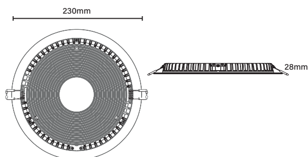
Opal Diffuser
