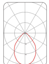
Low Glare Diffuser
