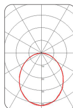
Opal Diffuser
